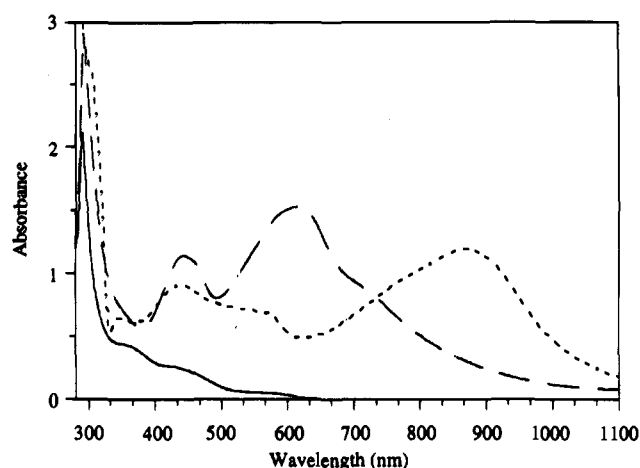
Figure 5. Spectrum of 12 , the reduction product of 7 , in (a) THF (—), (b) DMSO (---), and (c) THF/aqueous NaOH (- - -).
